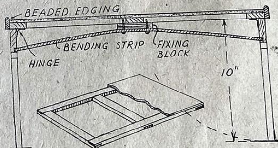
Fig. 2—Side section and detail of framework
