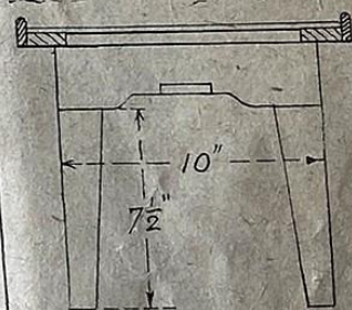
Fig. 3—End view, with legs open
